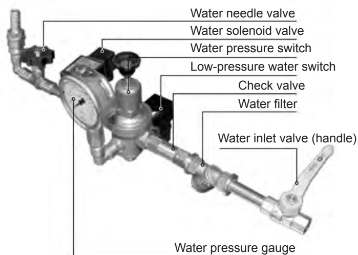
Water Train (.3 BTU/Hour)
