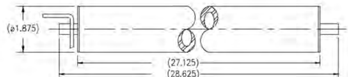
05-15180125 - No groove, with semi-precision bearing
