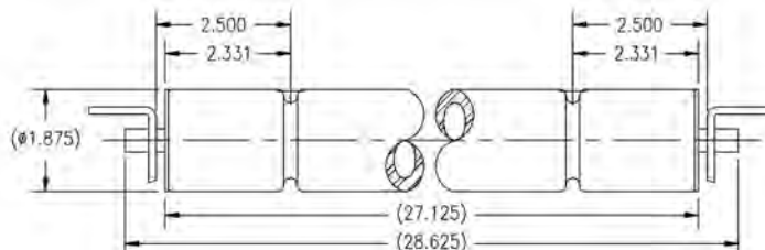
05-15180103 - Two grooves, opposite end
