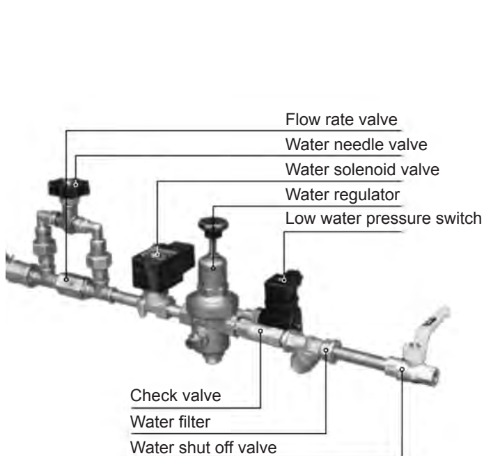
Water Train (.5 BTU/Hour)
