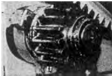
Fig. 1 - View of old style pinion
