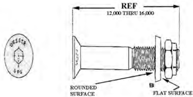
Flat Head Fastener
