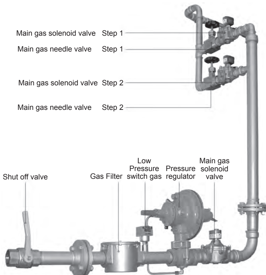
Fuel Train (Dual Speed/Variable Speed)
