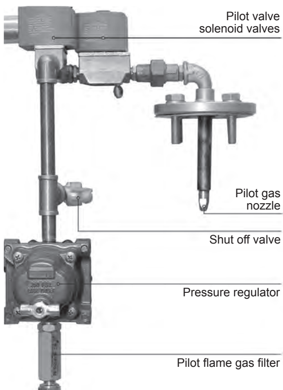
Pilot Flame Train (Dual Speed/Variable Speed)
