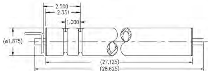
05-15180102 - Two grooves, common end
