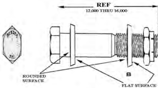
Hex Head Fastener
